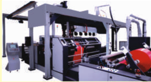
2 Extrusion Coating
